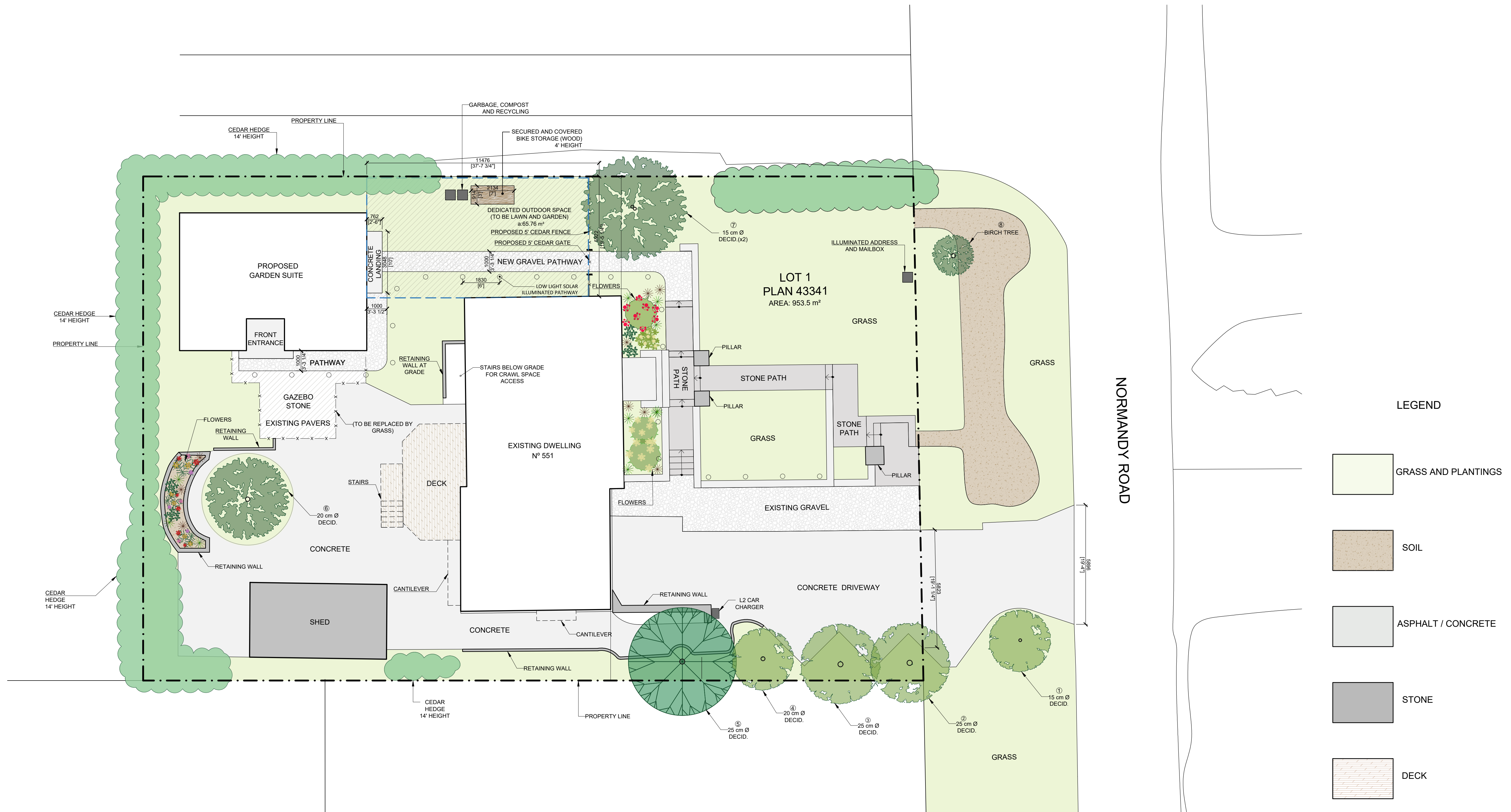
1 LANDSCAPE PLAN 1:100 0 4' 8' 16' 32'
