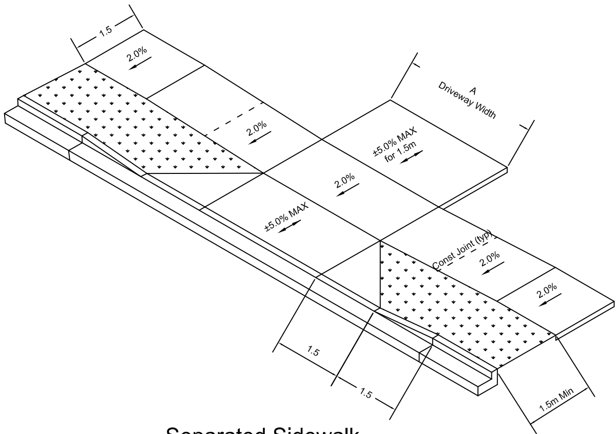
Separated Sidewalk
