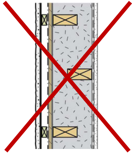
2x4 Double Stud Wall on 2x6 with Staggered Overlapping Studs (It is also nearly impossible to reach R-22 without a gap between the two stud walls)
