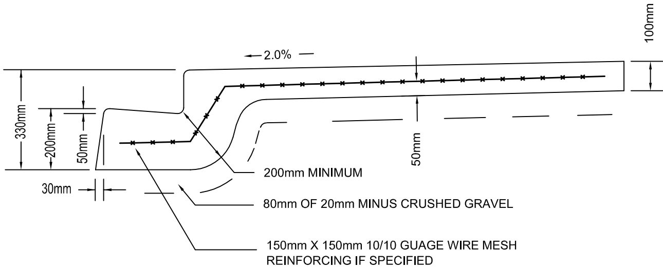
SIDEWALK SECTION
